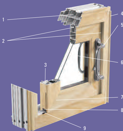
7500 Series Welded Sash
