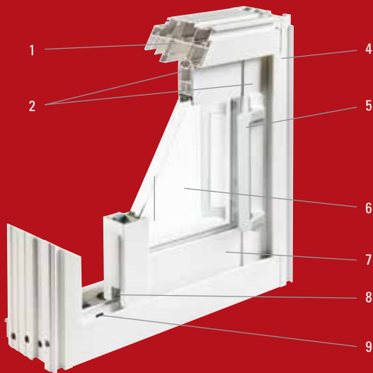
7800 Series Mechanical Sash
